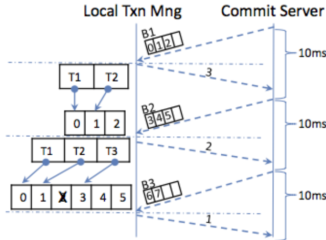
Figure 9: Proactive Commit Timestamp Management
