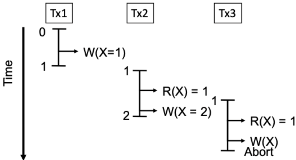
Figure 4: Snapshot Isolation in practice
