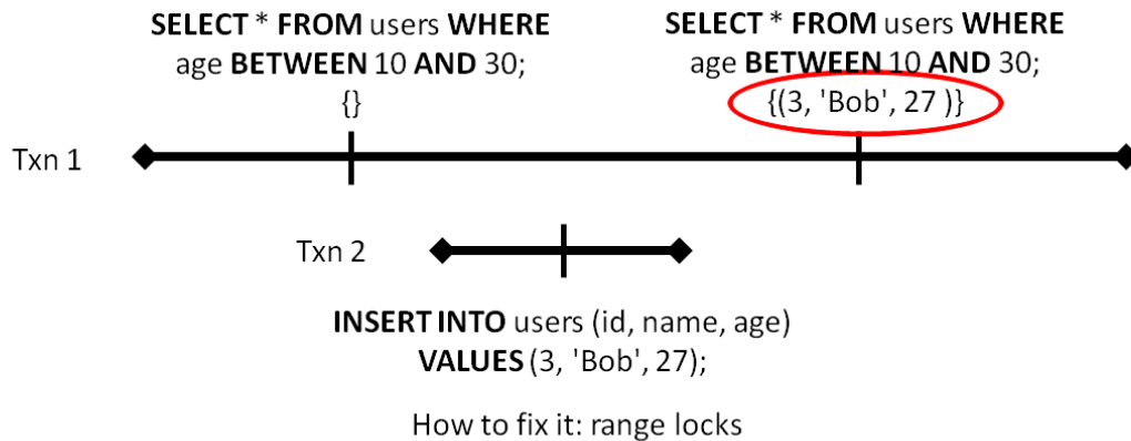
Figure 3: Phenomena: Phantom reads
