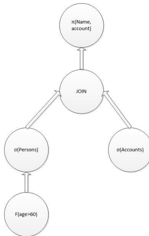
Figure 13: Alternative query plan
